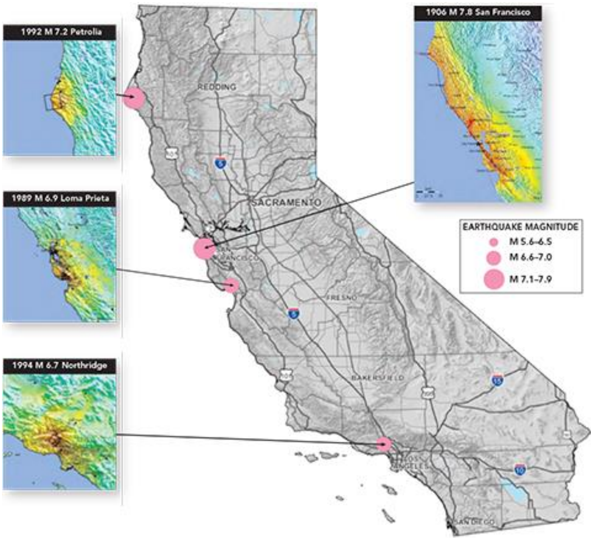
ShakeMap Explanation
